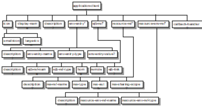
Figure 23. J2EE:application-client XML DTD Structure
