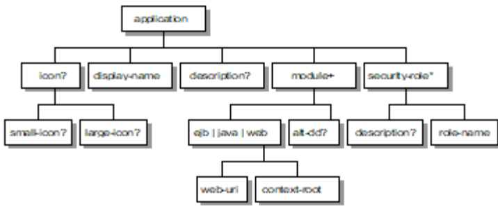
Figure 21. J2EE.application XML DTD Structure
