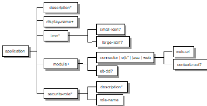
Figure 19. J2EE Application XML Schema Structure
