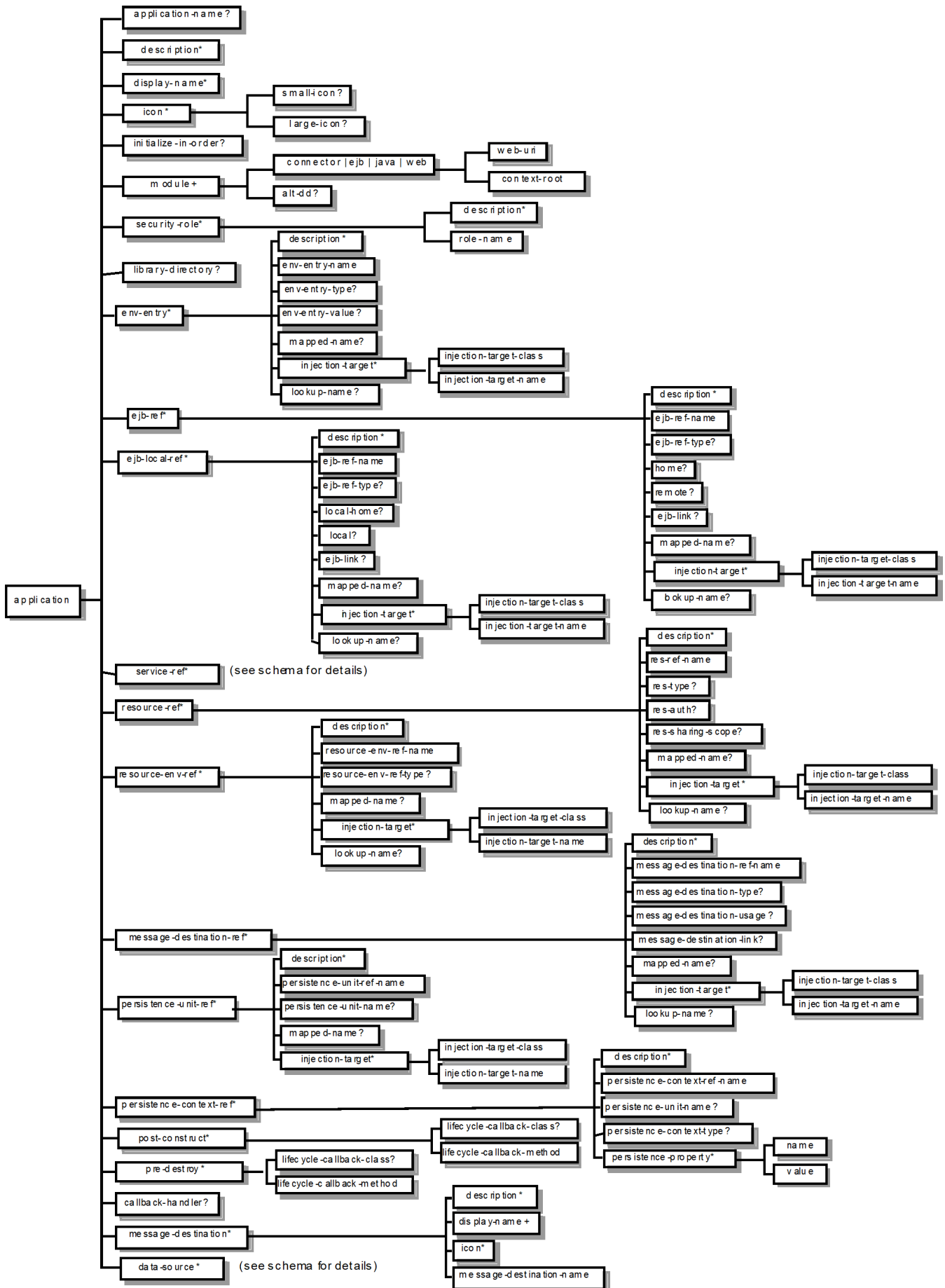
Figure 15. Java EE Application XML Schema Structure
