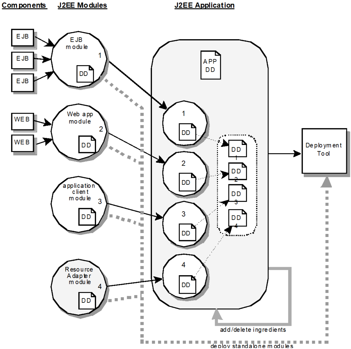
Figure 9. Jakarta EE Deployment
