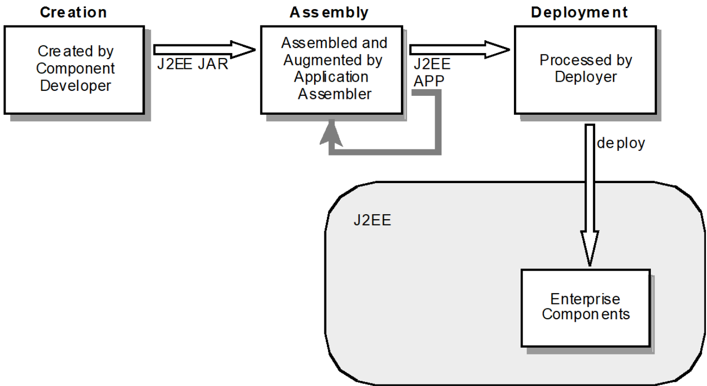
Figure 10. Jakarta EE Application Life Cycle
