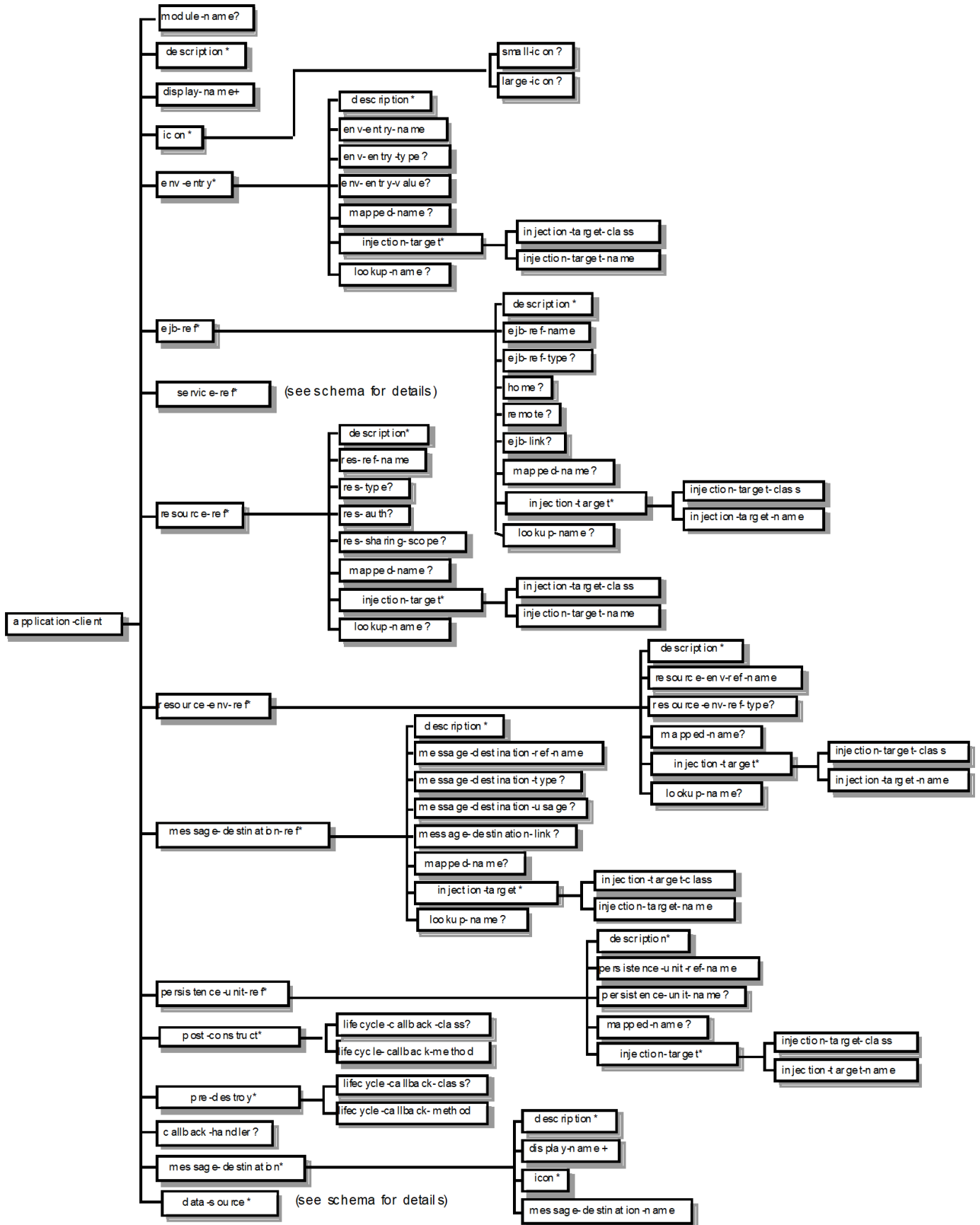
Figure 16. Java EE Application Client XML Schema Structure
