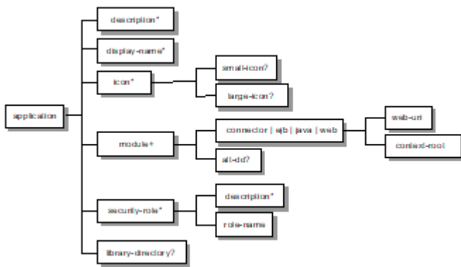
Figure 17. Java EE Application XML Schema Structure
