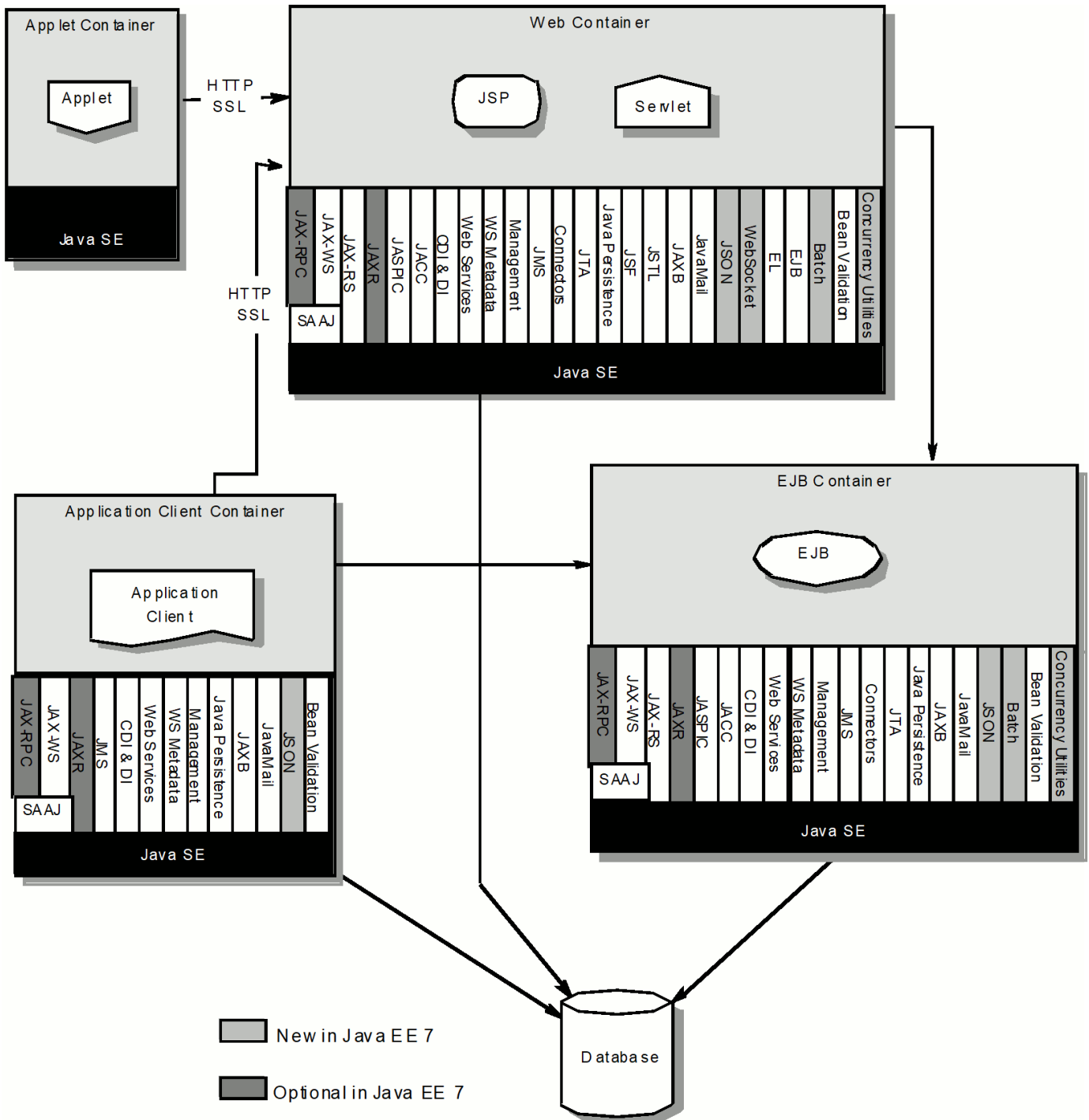
Figure 1. Jakarta EE Architecture Diagram
