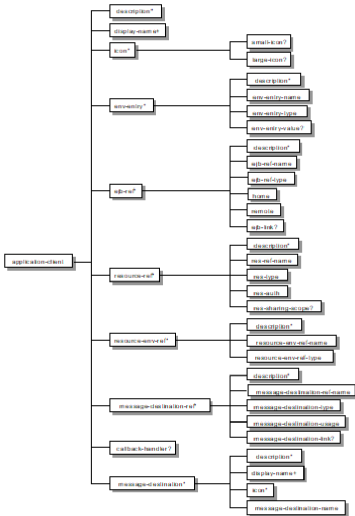
Figure 22. J2EE Application Client XML Schema Structure
