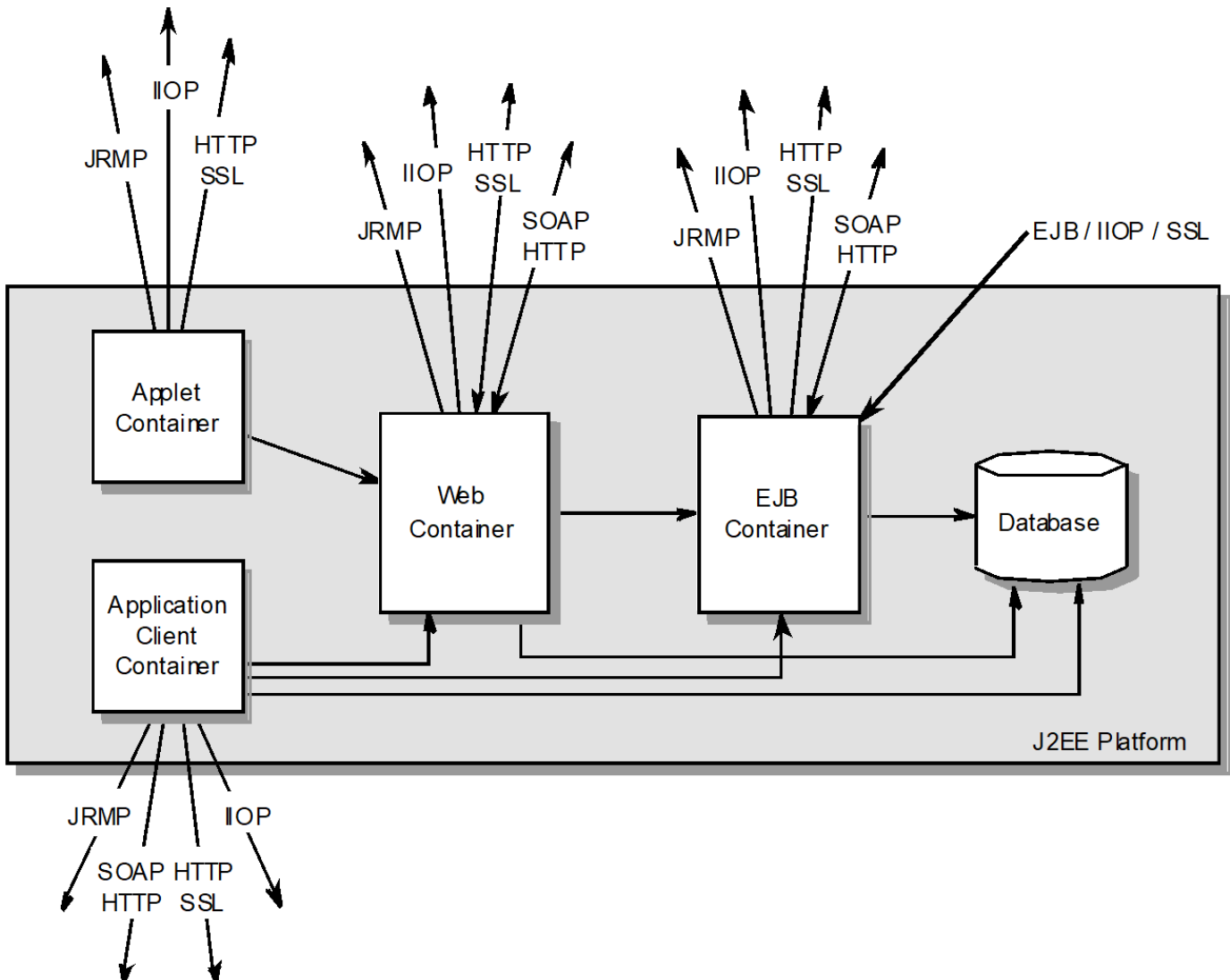
Figure 2. Java EE Interoperability
