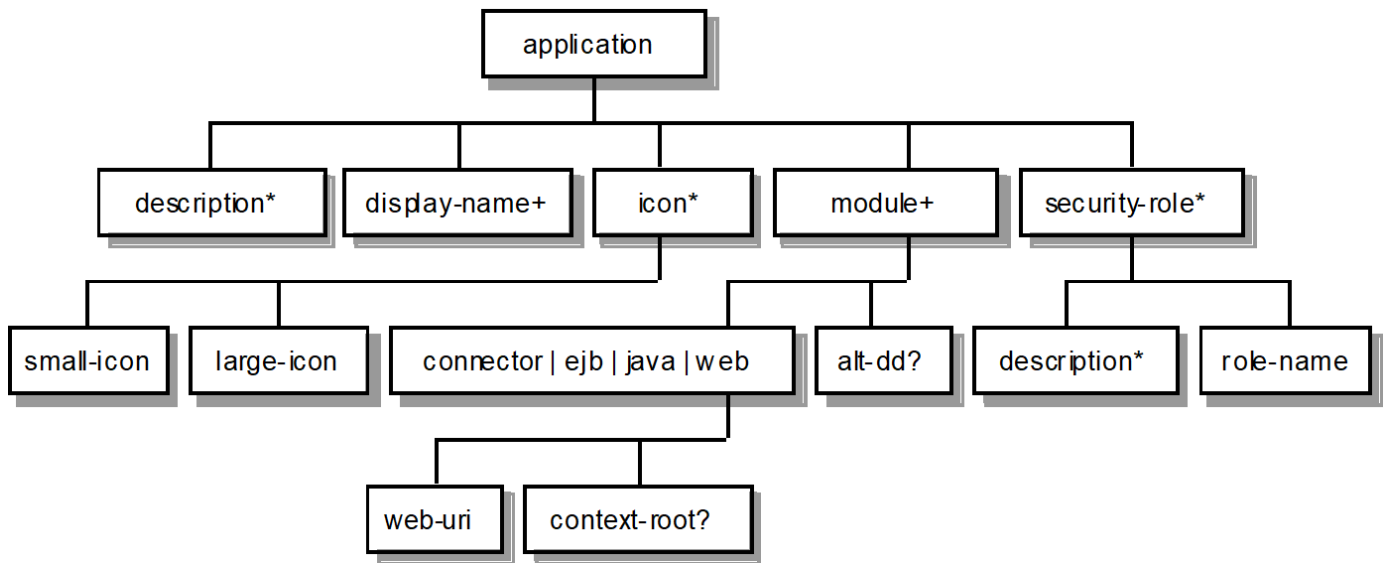
Figure 20. J2EE:application XML DTD Structure
