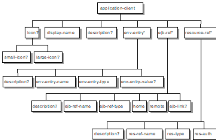
Figure 24. J2EE:application-client XML DTD Structure
